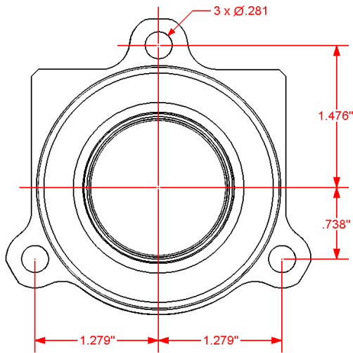
Figure 2: Bolt pattern of the Universal assembly
