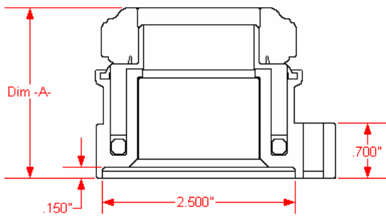
Figure 3: Side-view of Universal assembly
