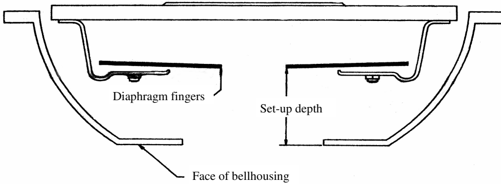
Figure 1: Set-up Depth Measurement
